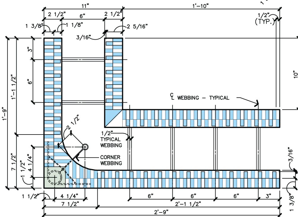
90° REVERSIBLE CORNER TOP / BOTTOM VIEW SCALE: 1 1/2" = 1'-0"
