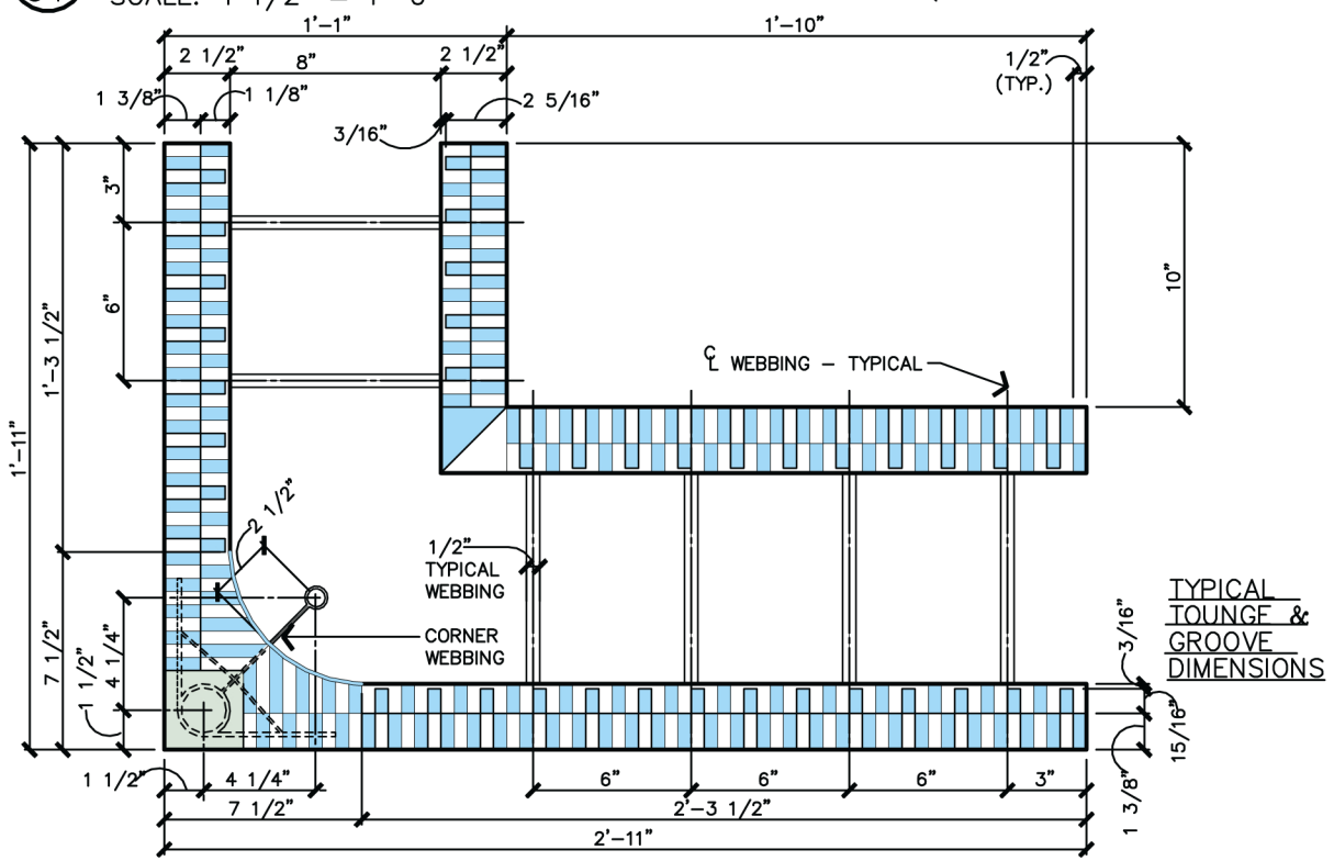
① ④ 90° REVERSIBLE CORNER TOP / BOTTOM VIEW SCALE: 1 1/2" = 1'-0"
